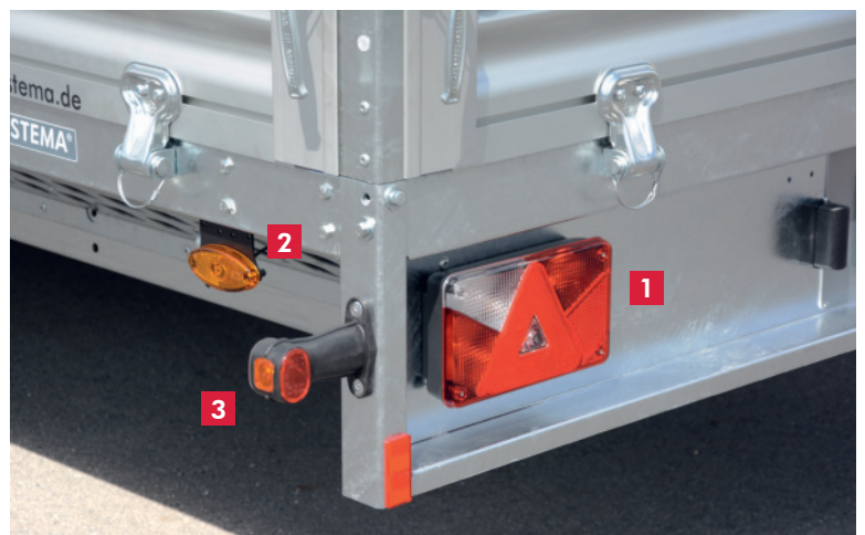
[1] Multipoint V lighting [2] side marker lights [3] clearance lights
